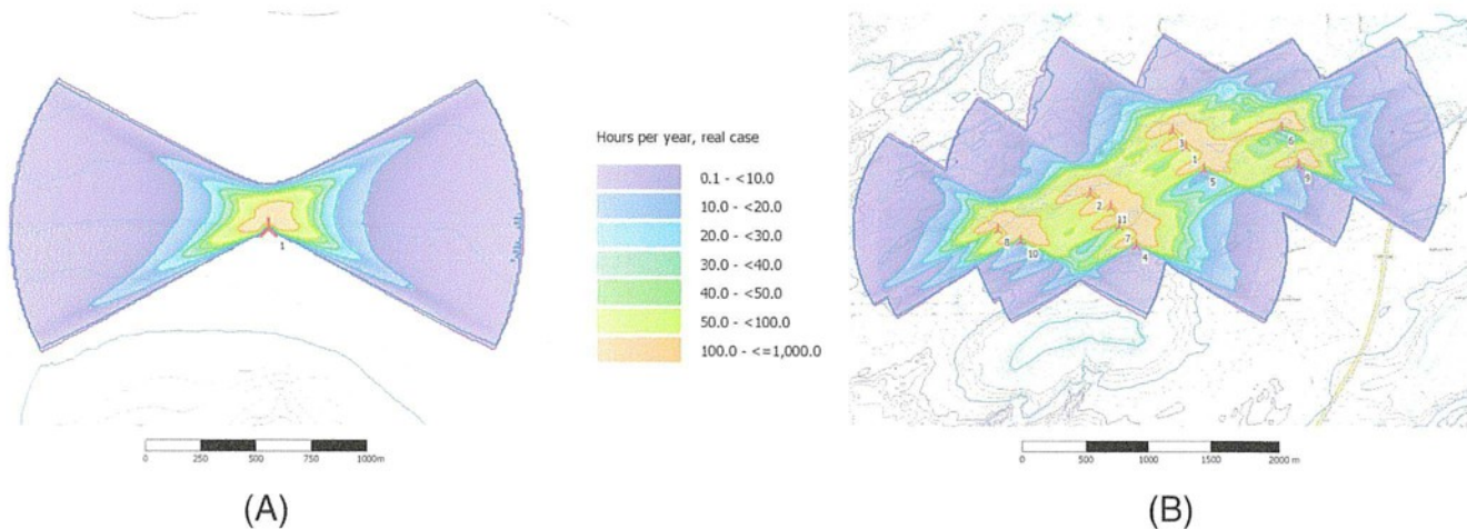
Fig. 2. Example of annual SF hours around (A) a single wind turbine and (B) a string of wind turbines.
